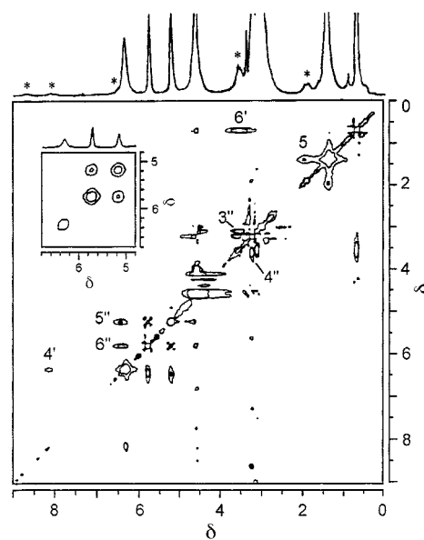
Fig. 5 The ^1\text{H} EXSY spectrum (360.13 MHz, 298 K, mixing time 20 ms) of the complex \text{Fe}^{2+} –SN in the presence of residual free drug (asterisked) in \text{CD}_3\text{OD} . The inset is a COSY spectrum showing the \text{H}5'' – \text{H}6'' through-bond coupling. The numbers indicate the assignment of the signals to the structure shown in Fig. 1
